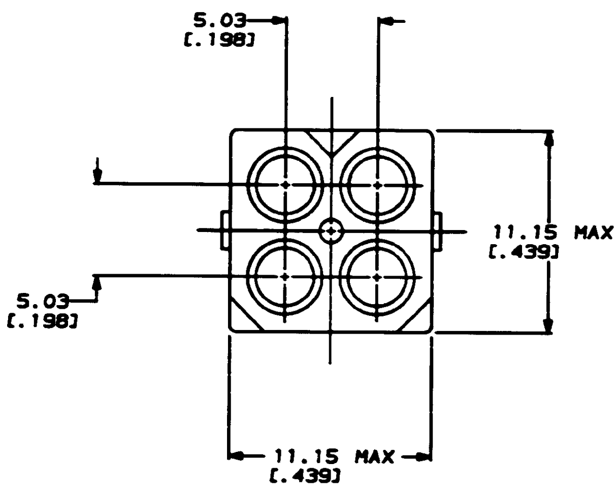
MATING CONNECTOR INTERFACE
